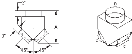
Standard "K" Valve
