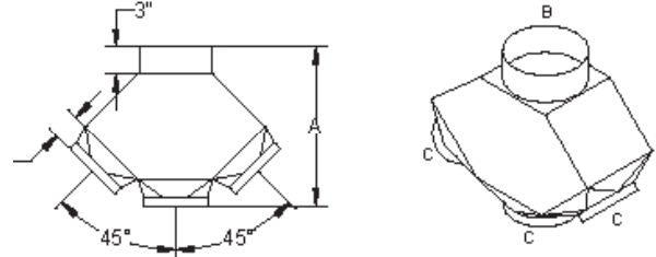
Standard 3-way Valve
